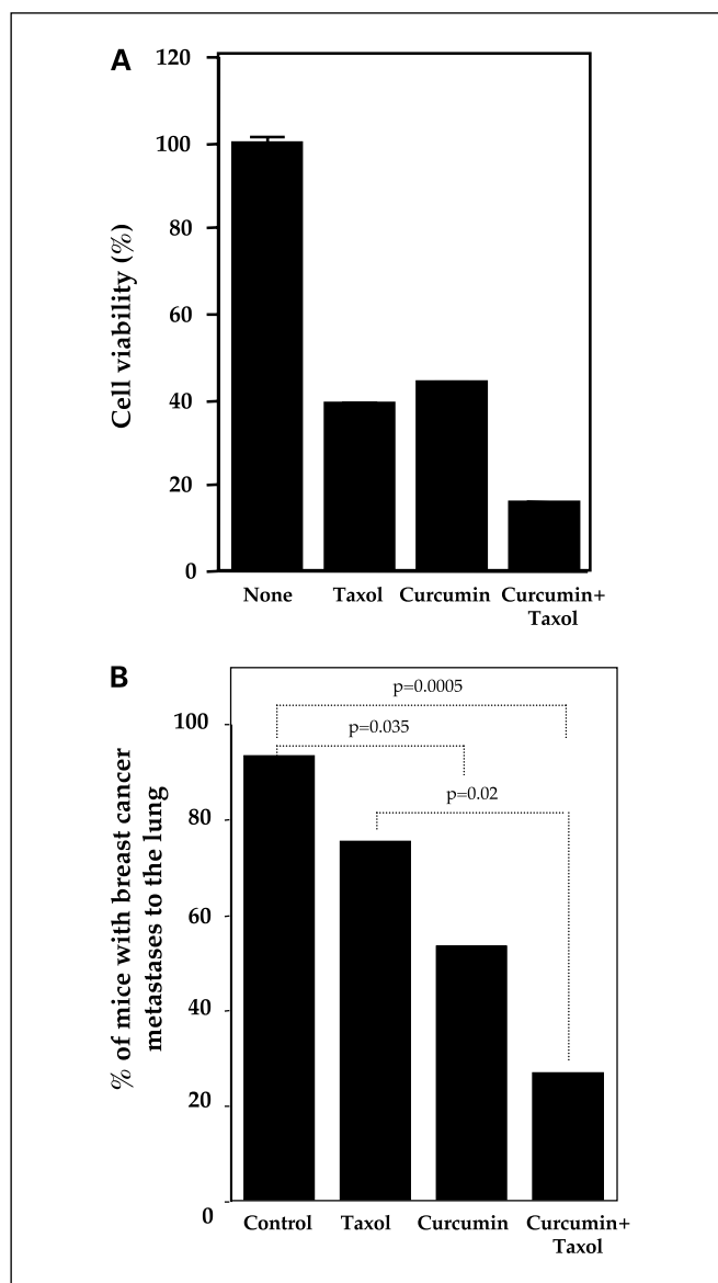
Fig. 5. A , curcumin potentiates the cytotoxic effects of paclitaxel against human breast cancer MDA-MB-435 cells. Cells (50,000/mL) were incubated in triplicate with either 50 \mu M/L curcumin or 10 \mu M/L paclitaxel or in combination for 72 hours, and then cell viability was measured by the 3-(4,5-dimethylthiazol-2-yl)-2,5-diphenyltetrazolium bromide method. B , curcumin, paclitaxel, and their combination inhibit breast cancer metastasis to the lung. Incidence of lung tumor metastasis was examined in mice after primary tumors were removed surgically. P values were determined using Fisher's exact test.
