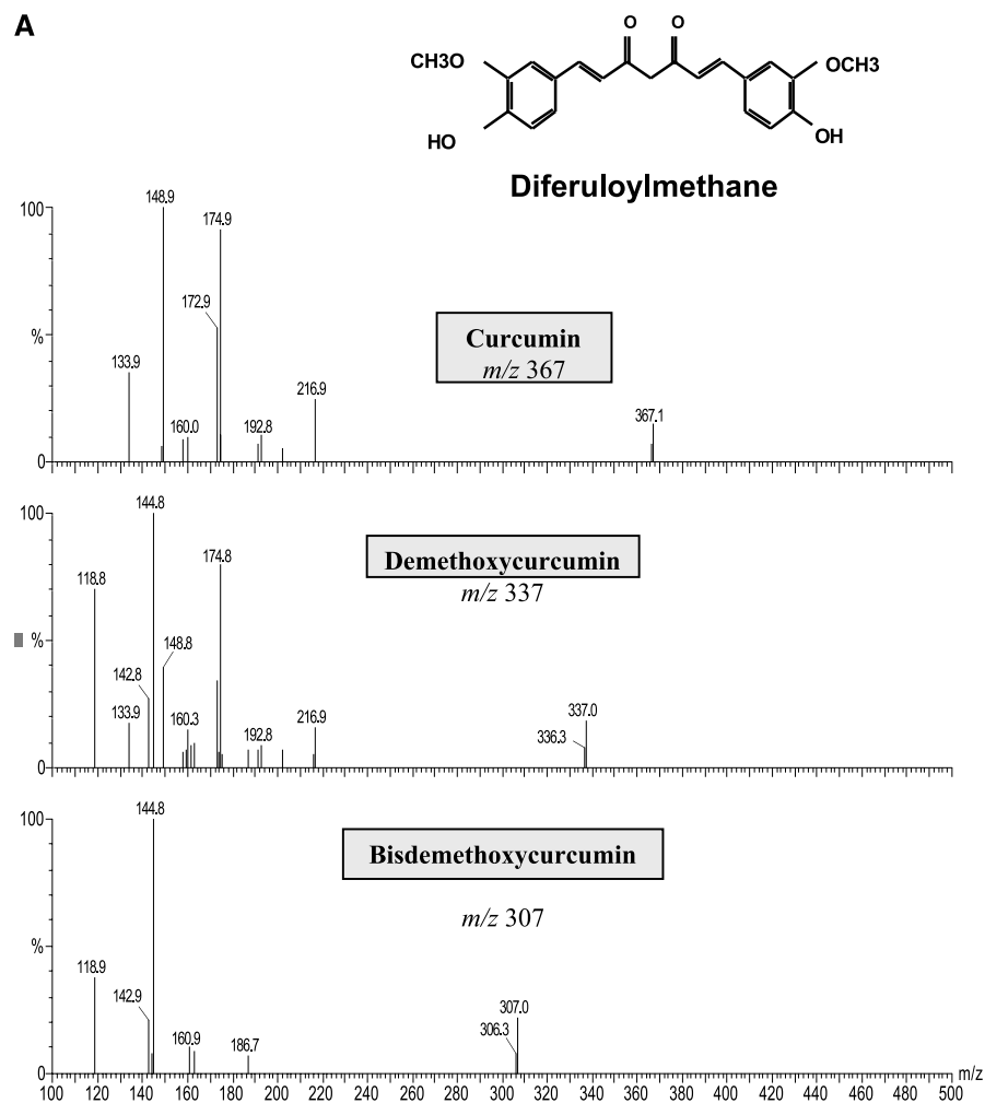
Fig. 1. A , structure and mass spectrophotometric analysis of curcumin. B , curcumin inhibited paclitaxel-dependent NF- \kappa B activation. MDA-MB-435 cells ( 2 \times 10^5 /mL) were preincubated with different concentrations of curcumin for 2 hours at 37°C and then treated with 50 \mu M paclitaxel for 16 hours. Nuclear extracts were prepared and tested for NF- \kappa B activation as described in Materials and Methods.
